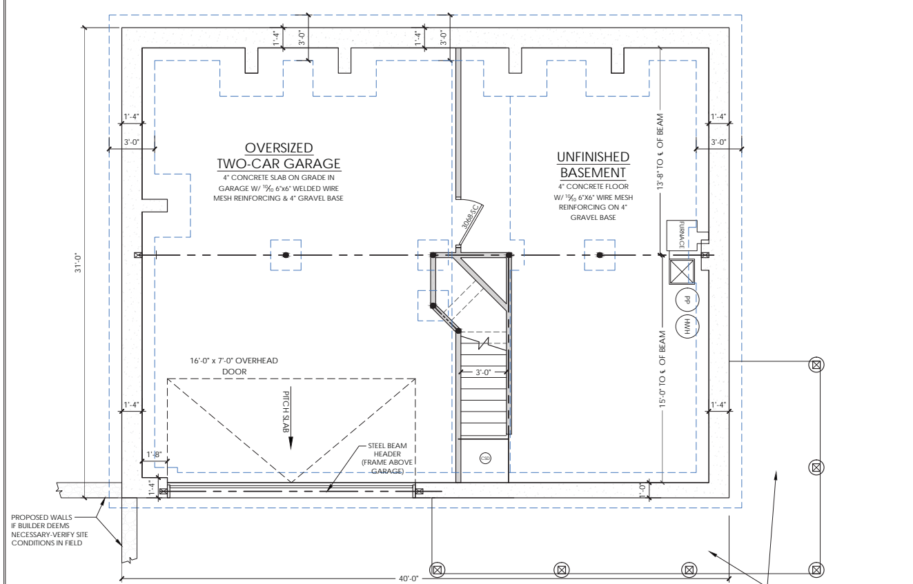
FOUNDATION FLOOR PLAN ① SCALE: 1/4" = 1'-0"
