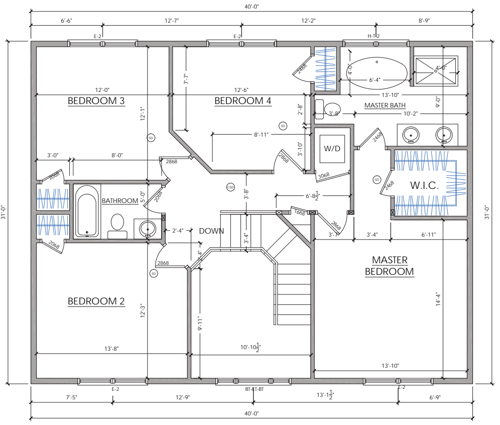
SECOND FLOOR PLAN ② SCALE: 1/4" = 1'-0"
